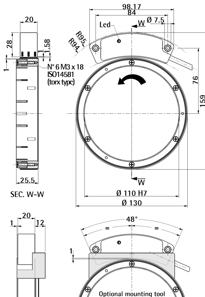
Figure 1 - Overall dimensions of the measuring system
