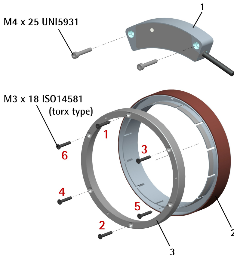
Figure 3 - Installing the ring
