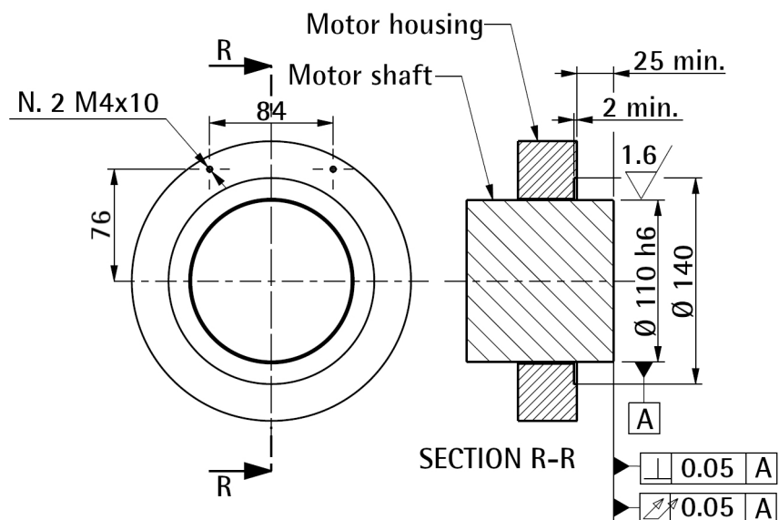
Figure 2 - Overall dimensions of the mounting support
